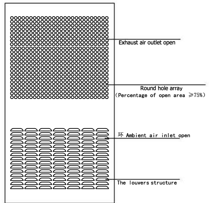
Figure 3-Installation Instruction
