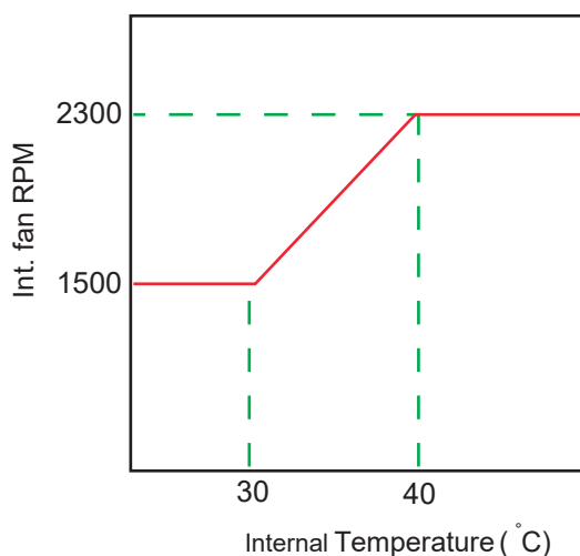
Int.Fan Speedvs.Cabinetinside temperature Curve
