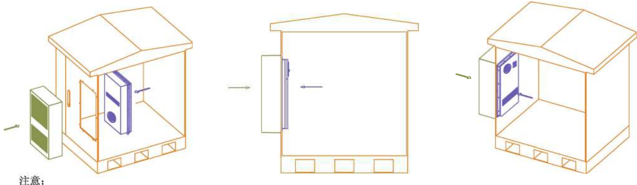
Figure 3-Installation Instruction
